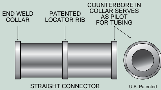
Figure 1 – The Automatic Buttweld fitting has a locator rib positioned a fixed distance from the end weld collar.
